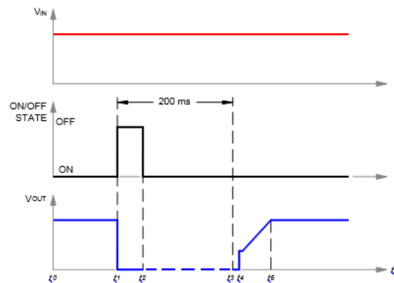
Figure 7. Startup scenario #3.
