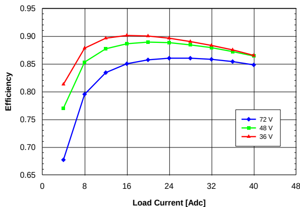
Figure 1.8V.11. Efficiency vs. load current and input voltage for QME48T40018 converter mounted horizontally with air flowing from pin 1 to pin 3 at a rate of 300 LFM (1.5 m/s) and T_a = 25\text{ }^{\circ}\text{C} .
