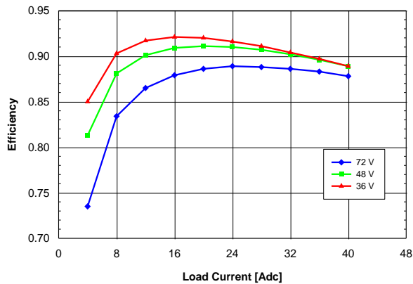
Figure 2.5V.11. Efficiency vs. load current and input voltage for QME48T40025 converter mounted horizontally with air flowing from pin 1 to pin 3 at a rate of 300 LFM (1.5 m/s) and T_a = 25^{\circ}\text{C} .
