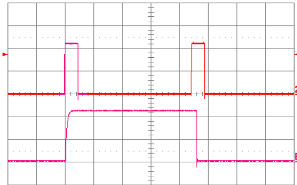
Figure 1.2V.24. Load current (top trace, 20 A/div., 50 ms/div.) into a 10 \text{ m}\Omega short circuit during restart, at V_{in} = 48 \text{ V} . Bottom trace (20 A/div., 5 ms/div.) is an expansion of the on-time portion of the top trace.
