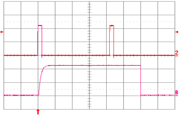
Figure 1.8V.24. Load current (top trace, 20 A/div., 50 ms/div.) into a 10 \text{m}\Omega short circuit during restart, at V_{in} = 48 \text{ V} . Bottom trace (20 A/div., 2 ms/div.) is an expansion of the on-time portion of the top trace.
