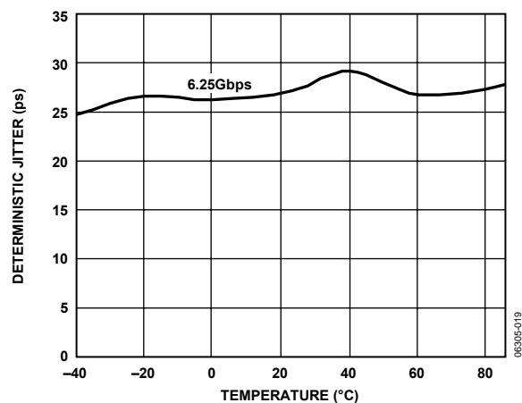
Figure 18. Deterministic Jitter vs. Temperature (Optimal EQ, 20" FR4)
