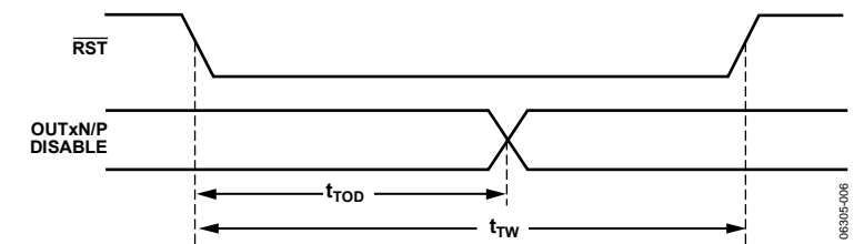
Figure 6. Asynchronous Reset
