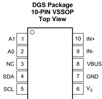
Pin Functions
