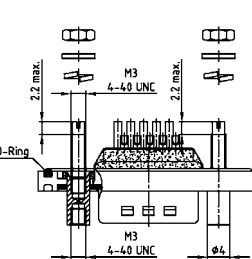
Mounting style: Front spacer and rear mounting stud
