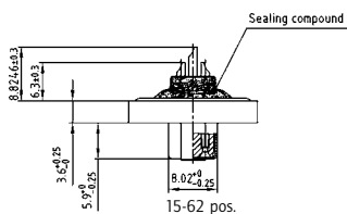
Mounting style: Front spacer and rear mounting stud
