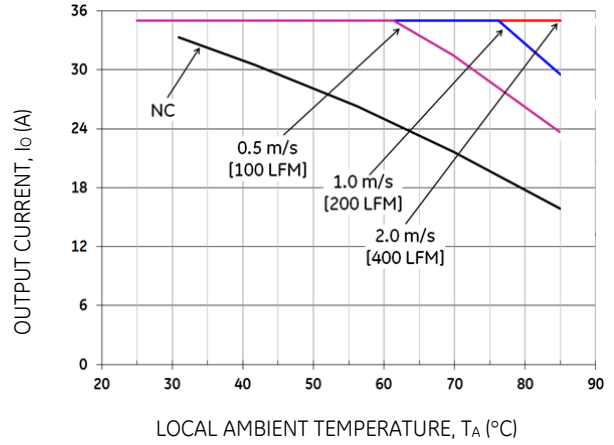
Figure 21. Output Current Derating for the Base plate QSDW035A0B-H with 0.5" heatsink in the Transverse Orientation; Airflow Direction from Vin(-) to Vin(+); Vin = 48V
