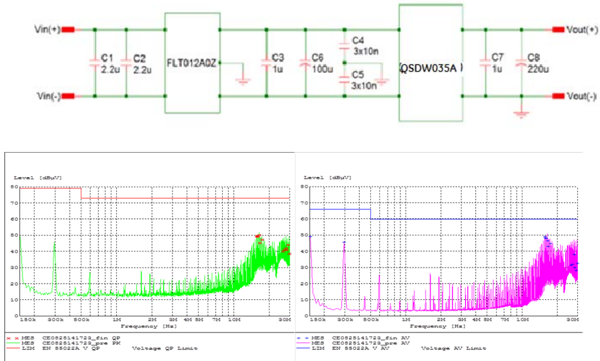
Figure 25. EMC Consideration
