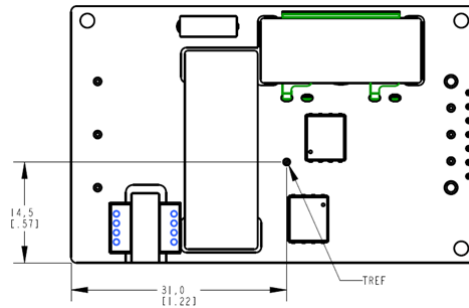
Figure 16. Location of the thermal reference temperature TH.
