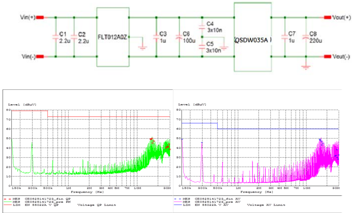
Figure 25. EMC Consideration
