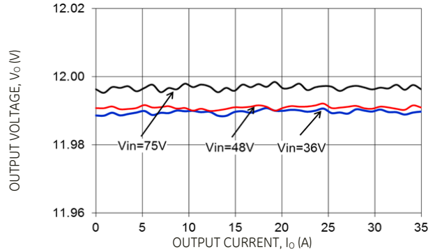
Figure 8. Typical Output Voltage Regulation vs. Output Current.
