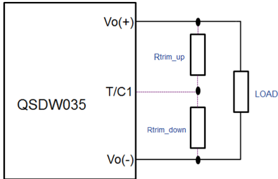
Figure 15. Circuit Configuration to Trim Output Voltage.
