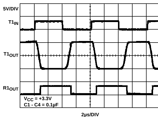
FIGURE 6. LOOPBACK TEST AT 250\text{kbps}
