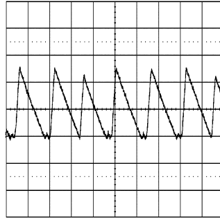
Figure 36. Transition Mode Operation V_{IN} = 24V , V_O = 3.3V , I_O = 0.35A 2 \mu\text{sec/div}
