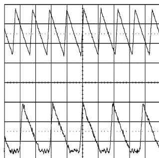
Figure 35. CCM and DCM Operating Modes V_{IN} = 24V , V_O = 3.3V , I_O = 2A/0.32A 2 \mu\text{sec/div}
