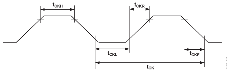
Figure 3. XTAL1 Input
