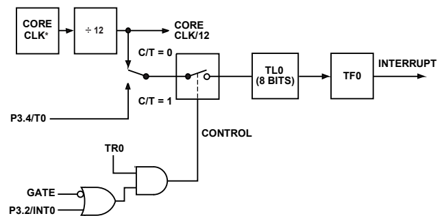
Figure 78. Timer/Counter 0, Mode 3
