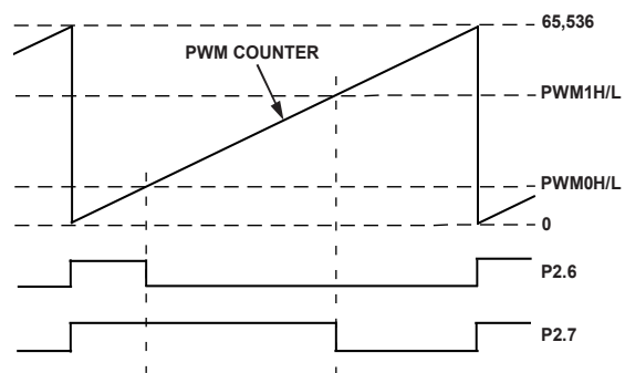
Figure 59. PWM Mode 3
