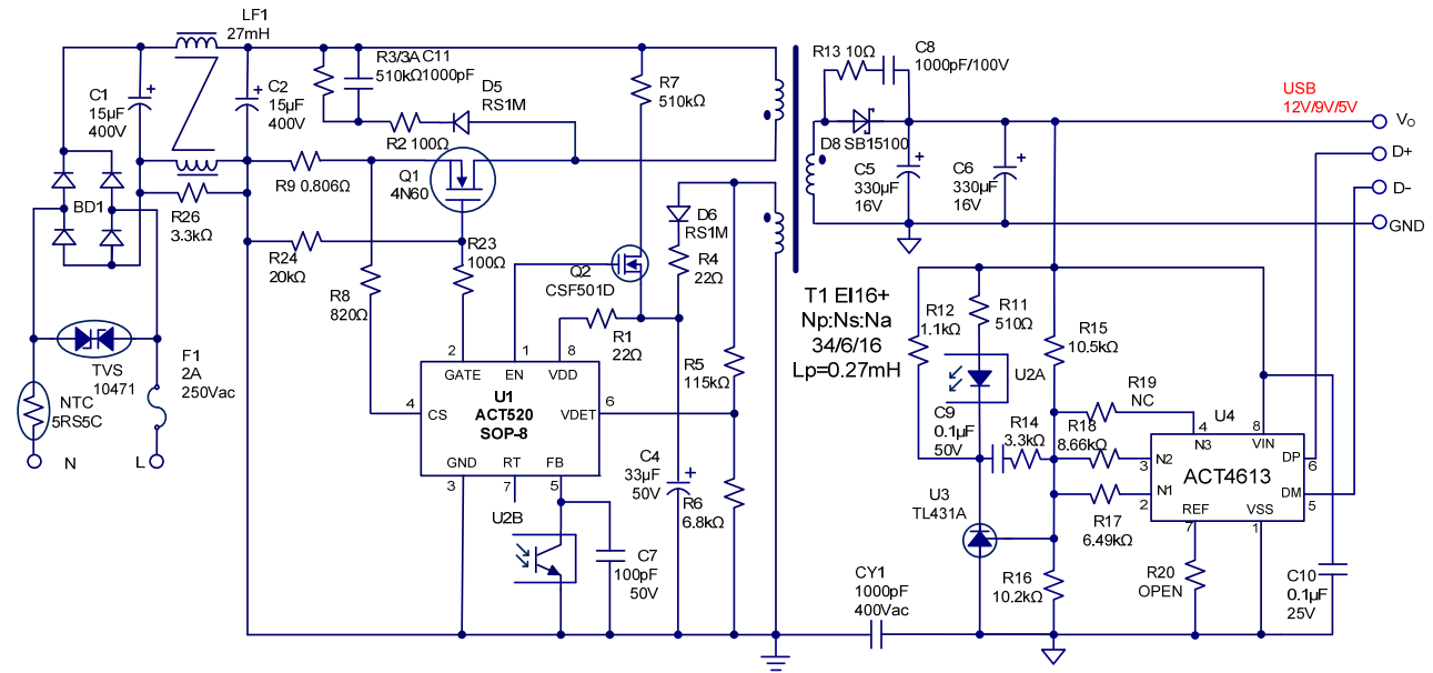
Figure 4: Universal VAC Input, 12/9/5V 1.5A rapid Charger
