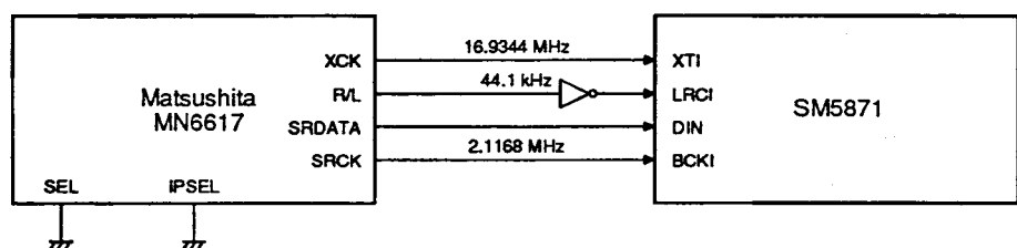
Figure 14. Matsushita MN6617 interface
