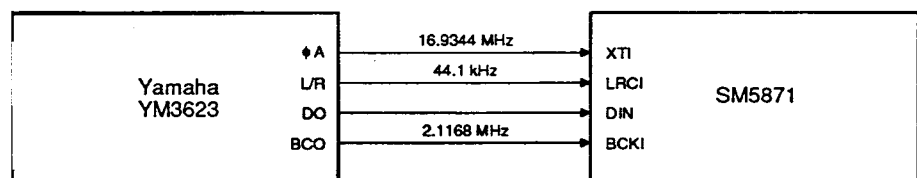
Figure 15. Yamaha YM3623 interface
