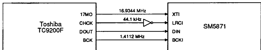
Figure 16. Toshiba TC9200F interface
