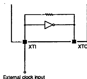
Figure 6. External system clock connection
