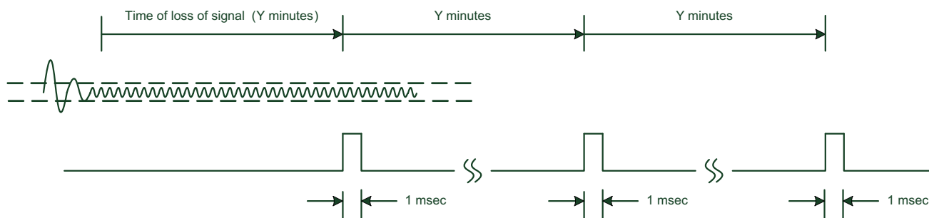
Figure 34. Interrupt Behavior for Signal Loss.
