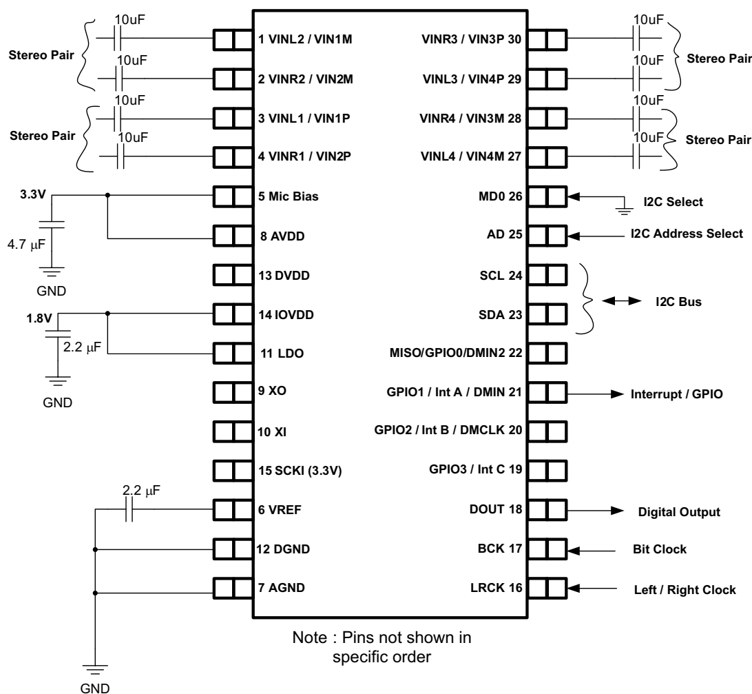
Figure 60. Simplified Schematic, PCM1862 I²C Controlled Subsystem
