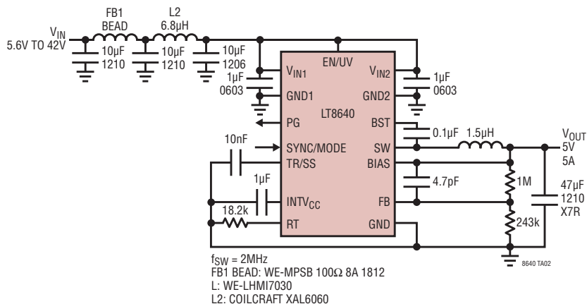
Ultralow EMI 5V, 5A Step-Down Converter
