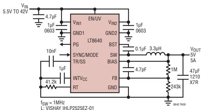
5V 5A Step-Down Converter
