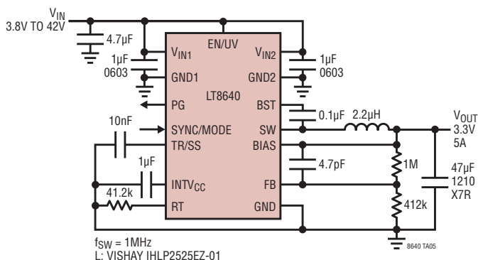
3.3V, 5A Step-Down Converter
