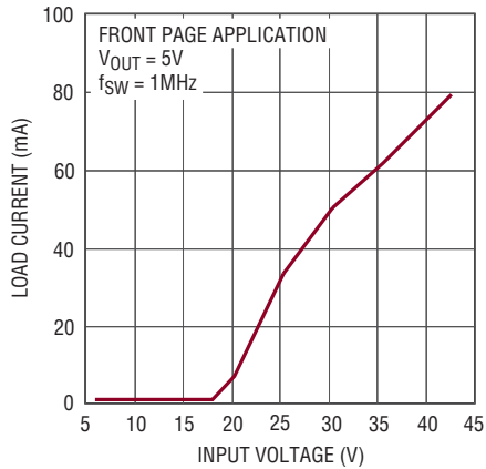
Minimum Load to Full Frequency (SYNC Float)
