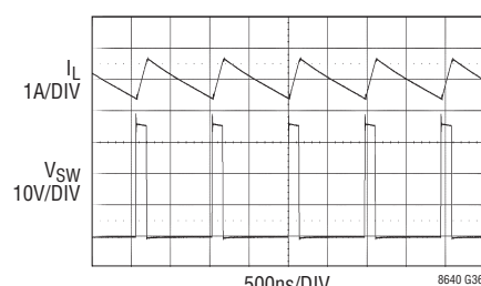
Switching Waveforms
