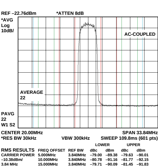
Figure 33. ACLR for Single WCDMA Carrier @ 20 MHz, f_{DATA} = 61.44 MSPS, 4x Interpolation
