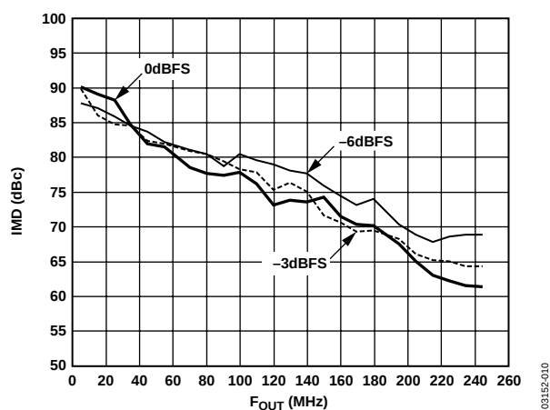
Figure 10. Out-of-Band SFDR, f_{DATA} = 125 MSPS, 4 \times Interpolation
