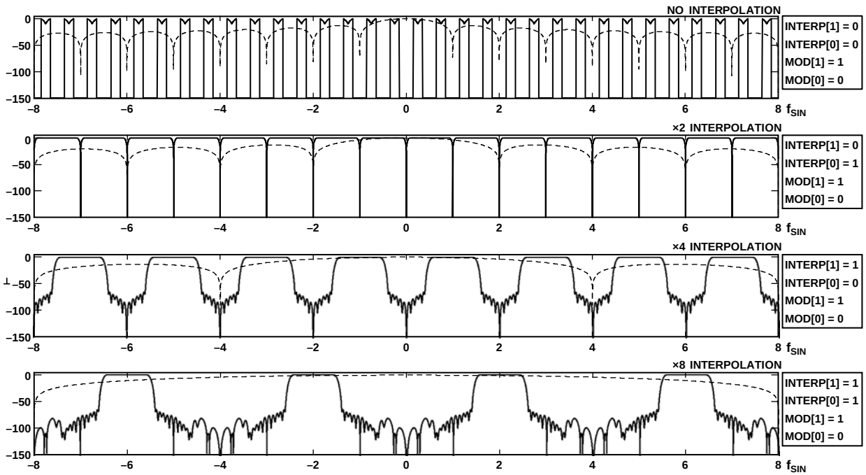
Figure 61. Real Modulation by f_{\text{DAC}}/4 Under All Interpolation Modes
