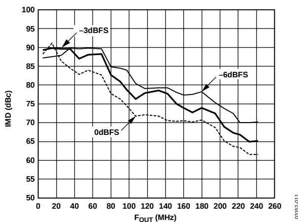
Figure 11. Out-of-Band SFDR, f_{DATA} = 62.5 MSPS, 8 \times Interpolation
