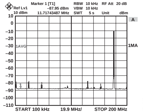
Figure 31. Two Tones Around 177 MHz, f_{DATA} = 200 \text{ MSPS} , 2x Interpolation, High-Pass Digital Filter Mode
