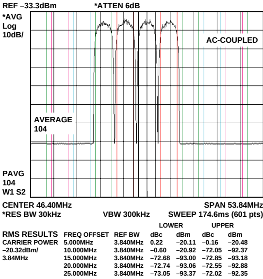
Figure 35. ACLR for Four WCDMA Carriers Near 50 MHz, f_{DATA} = 61.44 MSPS, 4x Interpolation
