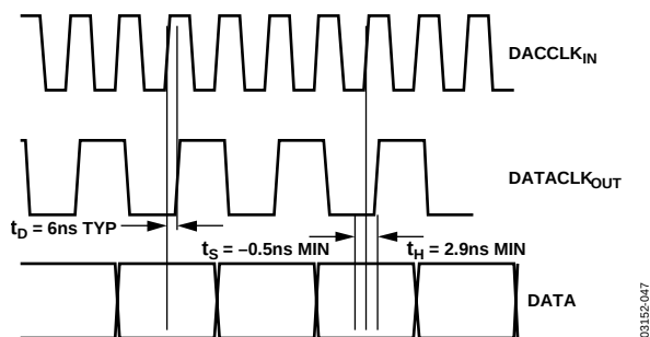
Figure 47. Data Timing, 2x Interpolation, DCLKPOL = 0
