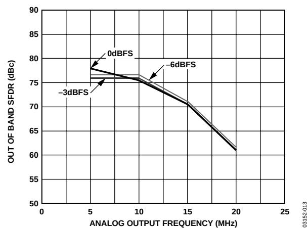
Figure 13. Out-of-Band SFDR, f_{DATA} = 50 MSPS, 8 \times Interpolation
