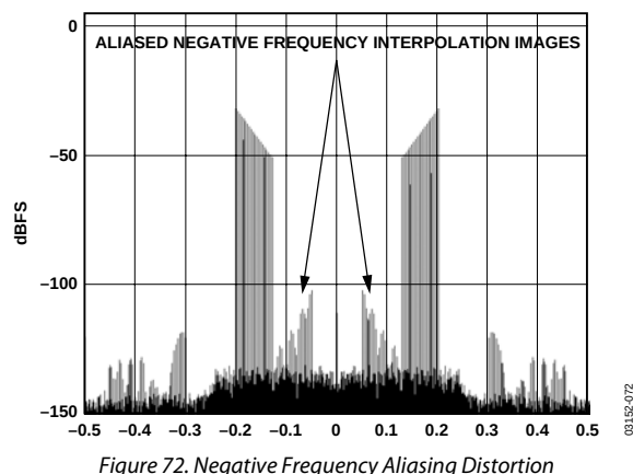
Figure 72. Negative Frequency Aliasing Distortion
