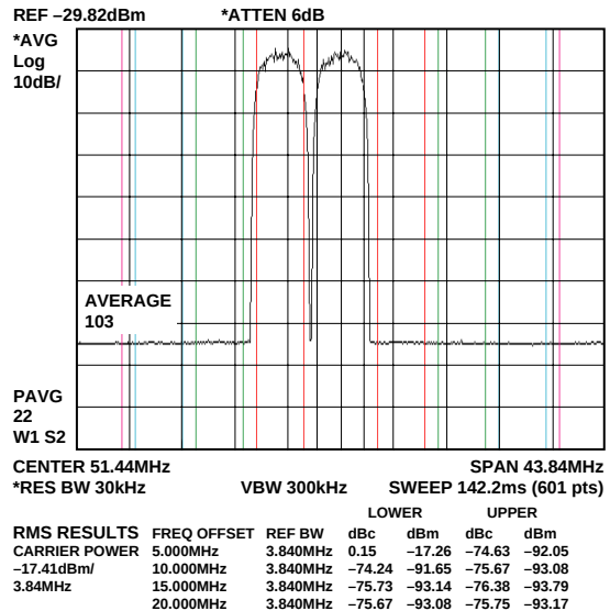
Figure 32. ACLR for Two WCDMA Carriers @ 51.44 MHz, f_{DATA} = 61.44 \text{ MSPS} , 4x Interpolation
