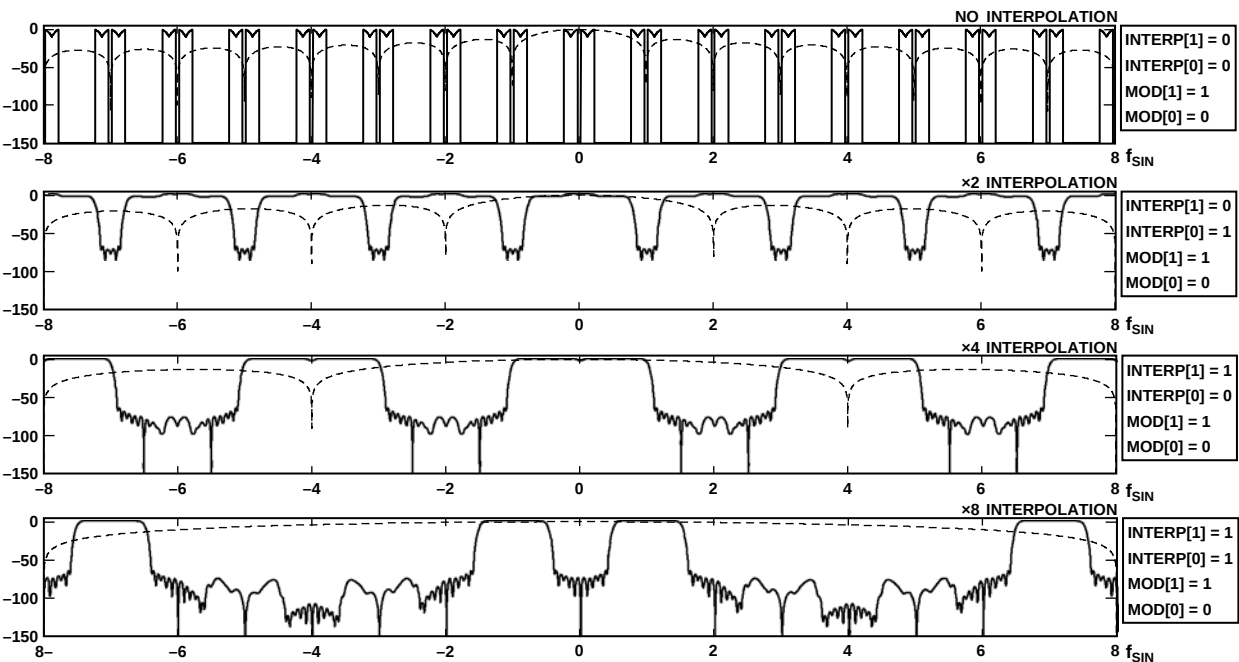
Figure 62. Real Modulation by f_{\text{DAC}}/8 Under All Interpolation Modes
