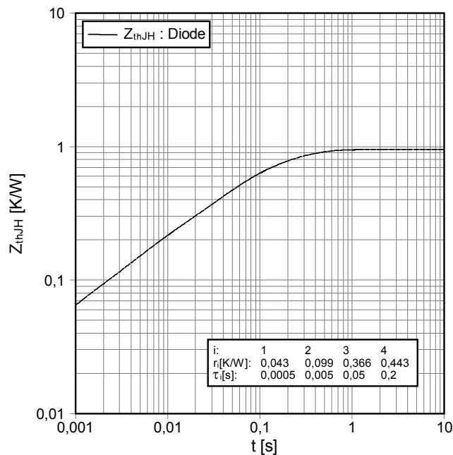
Transienter Wärmewiderstand Diode D5 - D6 transient thermal impedance Diode D5 - D6 Z_{thJH} = f(t)
