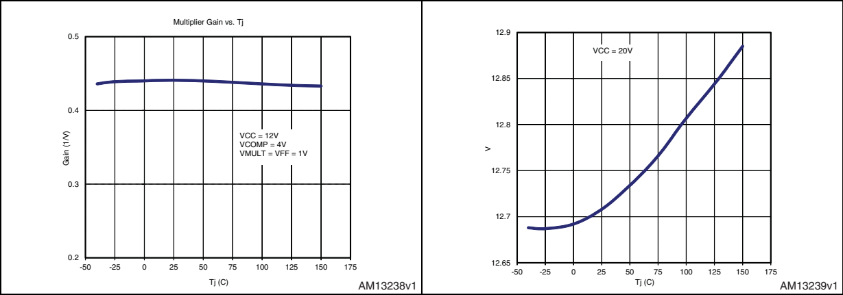
Figure 22. Multiplier gain vs. T_j Figure 23. Gate drive clamp vs. T_j
