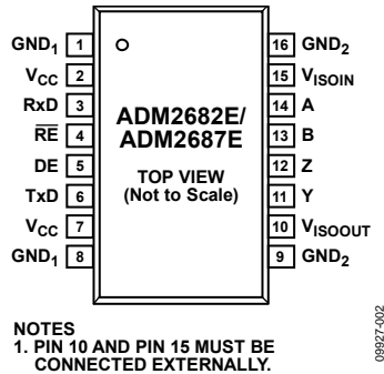
Figure 2. Pin Configuration
