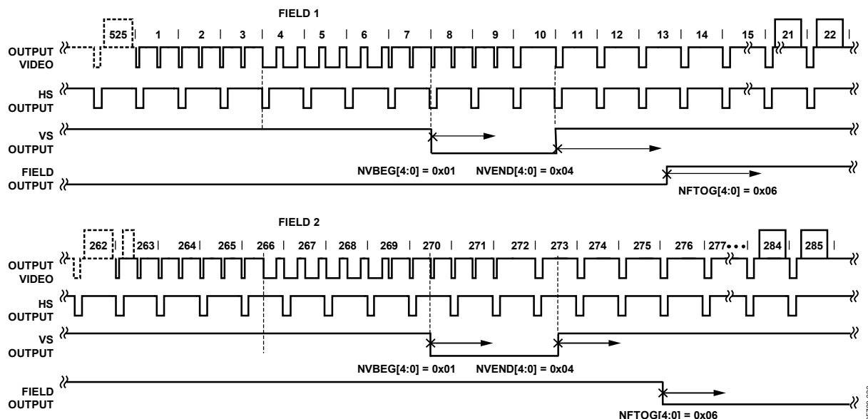
Figure 37. NTSC Typical VSYNC/FIELD Positions Using the Register Writes in Table 65
