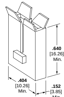
Cavity Part Number 1601470
