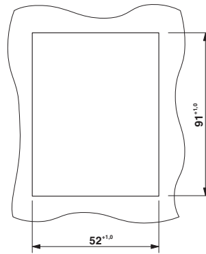
Dimensioned drawing
