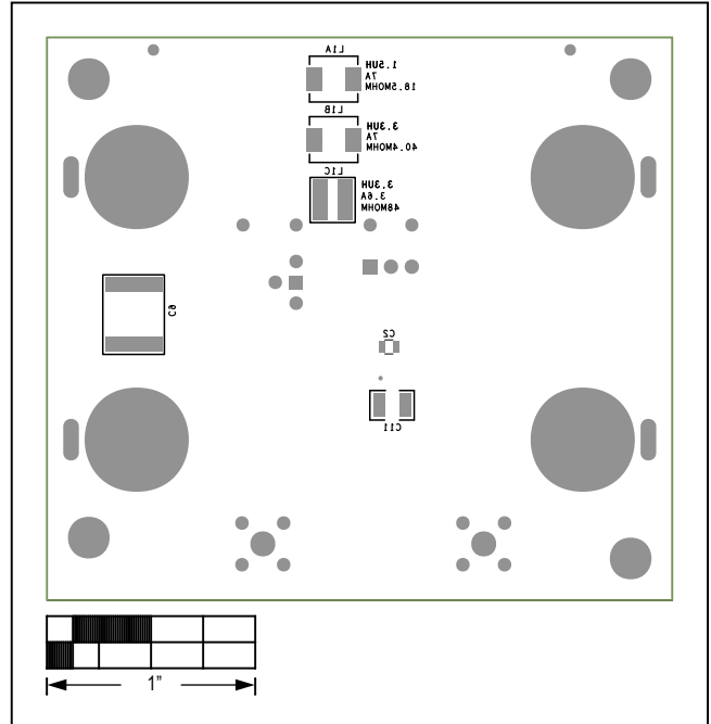
MAX17250 WLP EV Kit—Bottom Silkscreen
