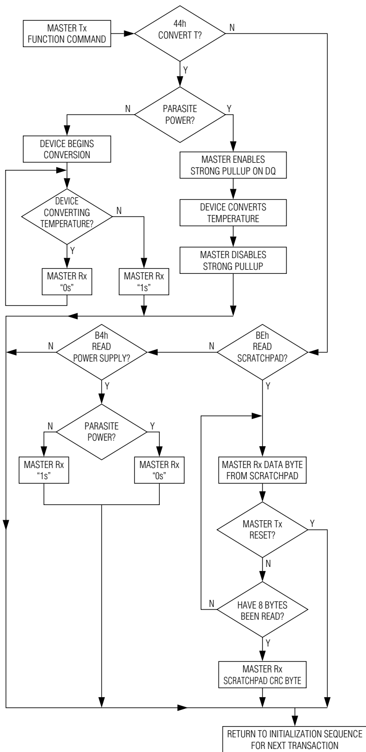
Figure 8. MAX31850/MAX31851 Function Commands Flowchart
