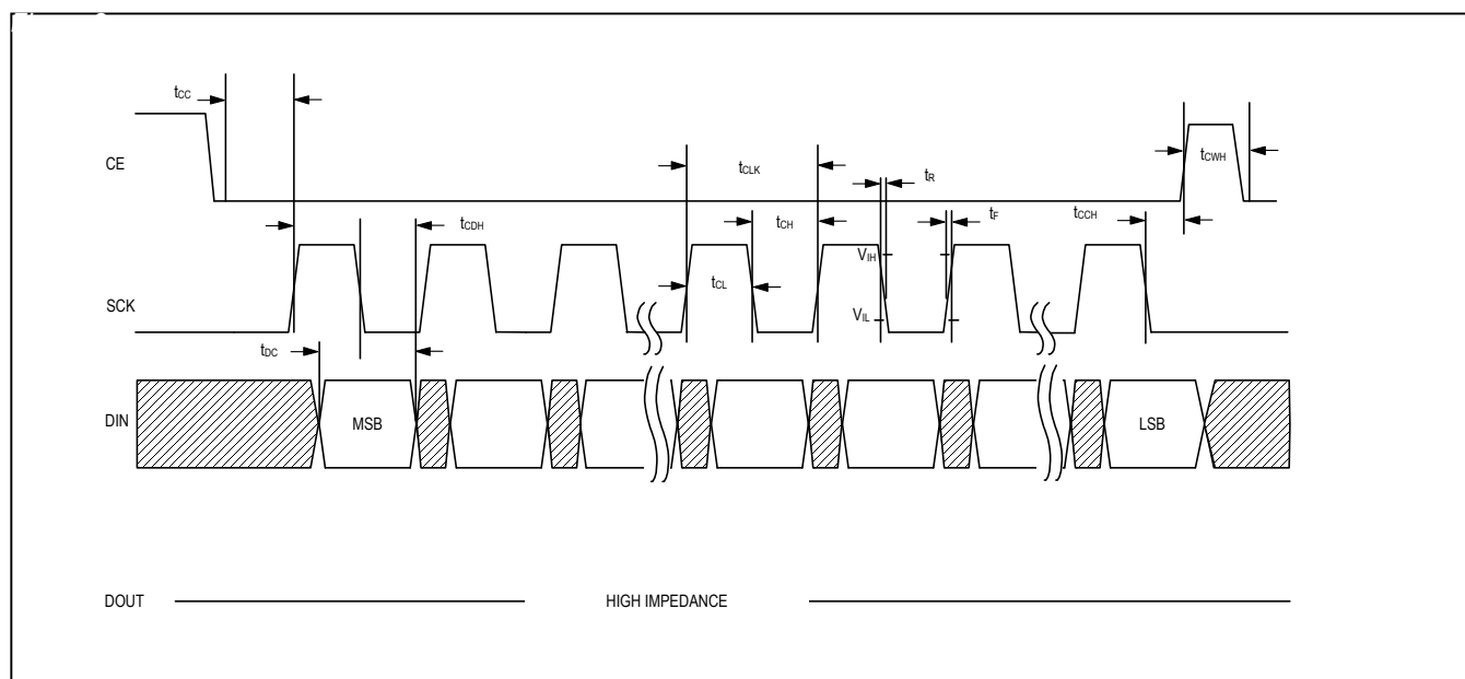
Figure 2. SPI Timing Diagram Write
