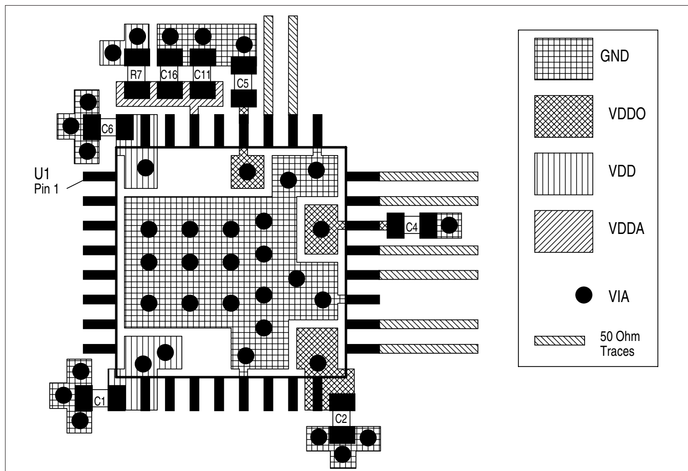
FIGURE 5B. PCB BOARD LAYOUT FOR ICS8745B
