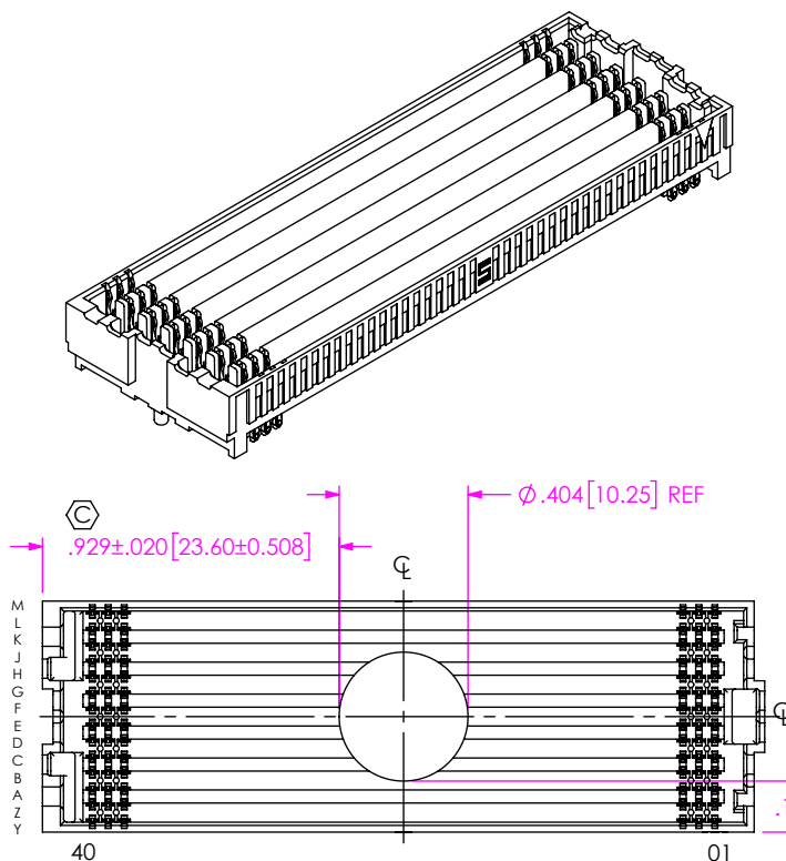
PAD &amp; VITA 57.4 DETAIL
