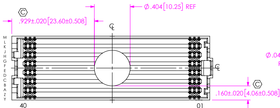
PAD &amp; VITA 57.4 DETAIL
