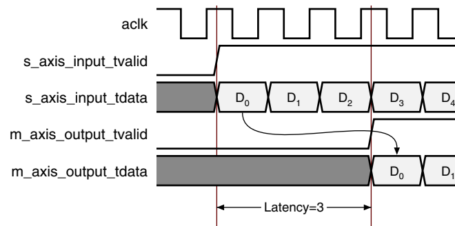
Figure 2-3: Latency
