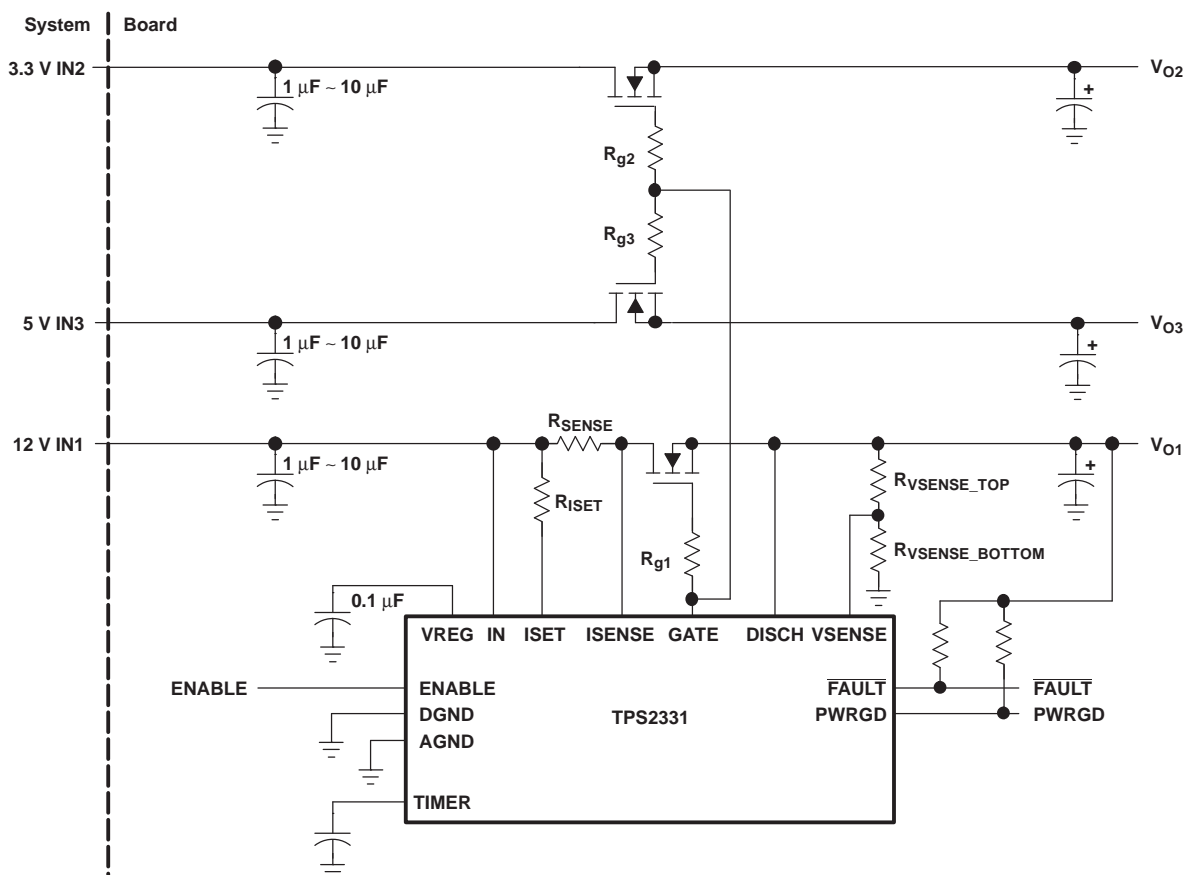
Figure 19. Three-Channel Application
