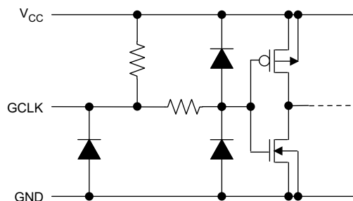
Figure 13. GCLK
