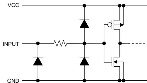
Figure 11. SIN, SCLK
