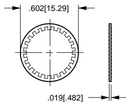
LOCKWASHER NICKEL-PLATED - 728-15907
