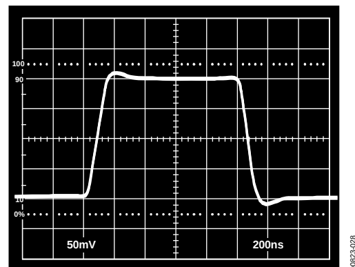
Figure 28. Unity-Gain Inverter Pulse Response (Small Signal)
