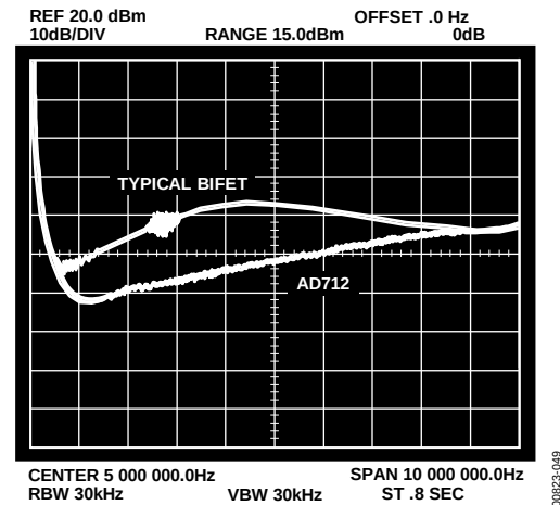
Figure 49. High Frequency Feedthrough
