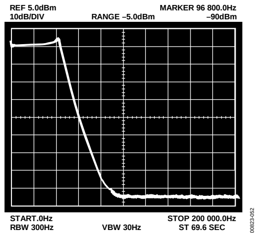
Figure 52. High Frequency Response for 9-Pole Chebychev Filter
