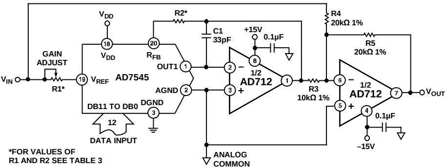
Figure 40. Bipolar Operation
