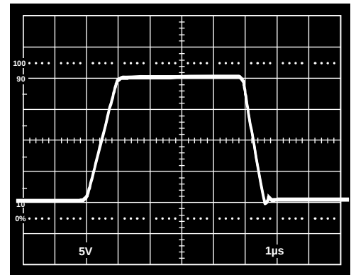
Figure 24. Unity-Gain Follower Pulse Response (Large Signal)
