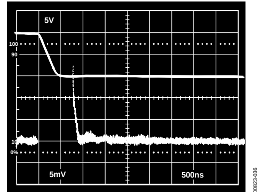
Figure 36. Settling Characteristics 0 V to -10 V Step Upper Trace: Output of AD712 Under Test (5 V/Div) Lower Trace: Amplified Error Voltage (0.01%/Div)
