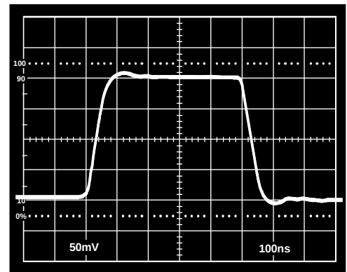
Figure 25. Unity-Gain Follower Pulse Response (Small Signal)
