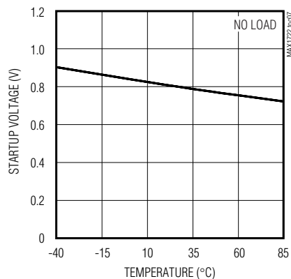
STARTUP VOLTAGE vs. TEMPERATURE
