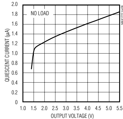
QUIESCENT CURRENT INTO OUT vs. OUTPUT VOLTAGE
