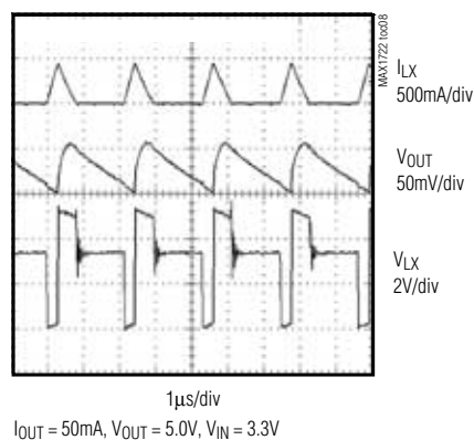
SWITCHING WAVEFORMS
