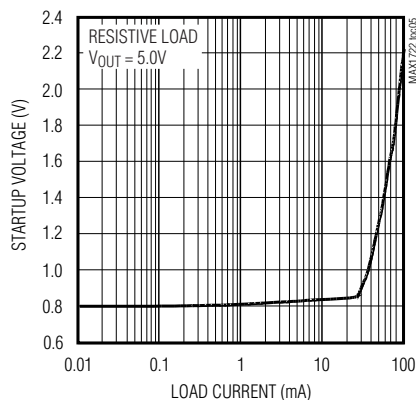
STARTUP VOLTAGE vs. LOAD CURRENT
