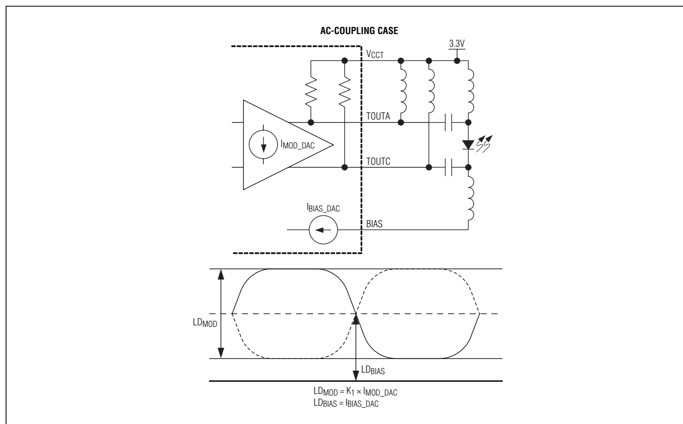
Figure 3. AC-Coupling Case
