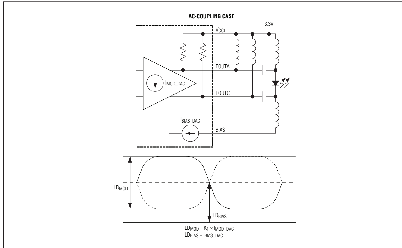
Figure 3. AC-Coupling Case
