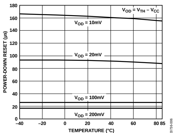
Figure 7. Power-Down Reset Delay vs. Temperature, ADM8xxT/S/R/Z
