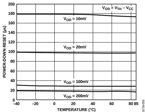
Figure 6. Power-Down Reset Delay vs. Temperature, ADM8xxL/M/J
