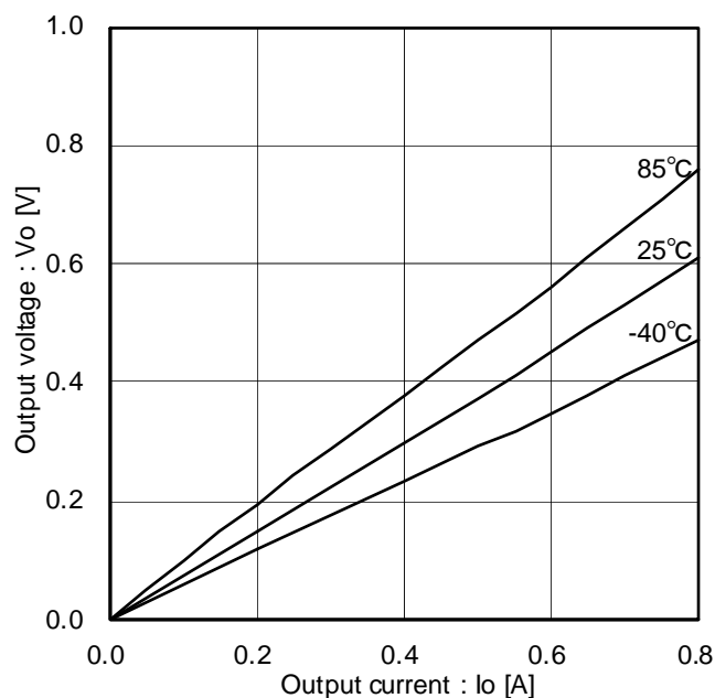
Figure 12. Output voltage (Upper and lower total) (Temperature characteristics)
