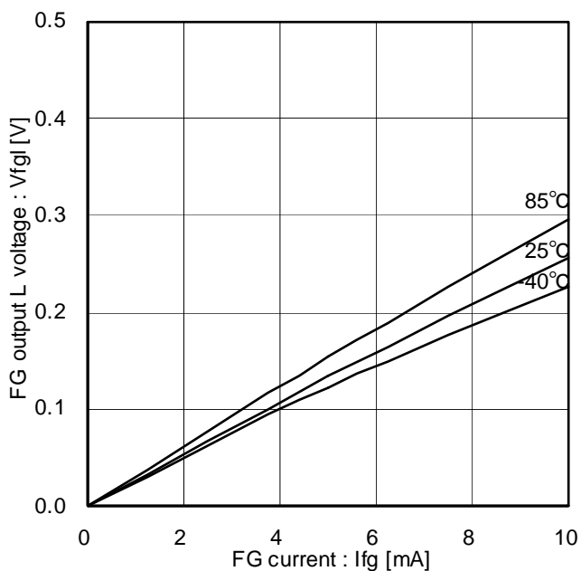
Figure 14. FG output L voltage (Temperature characteristics)
