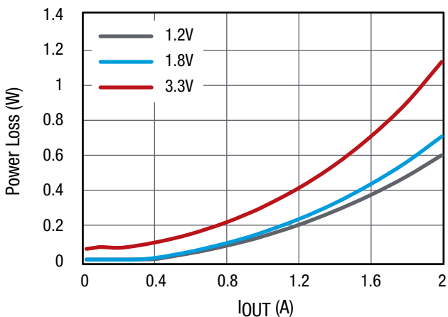
Figure 24. Channel 1 Power Loss at f sw = 500kHz, V IN = 5V, No Airflow
