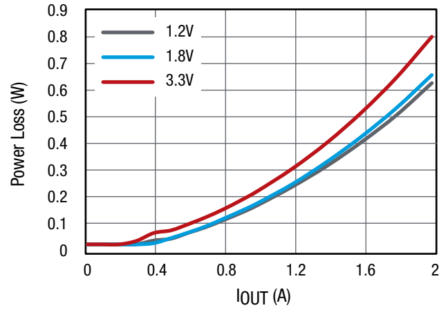
Figure 23. Channel 3 Power Loss at f sw = 500kHz, V IN = 12V, No Airflow
