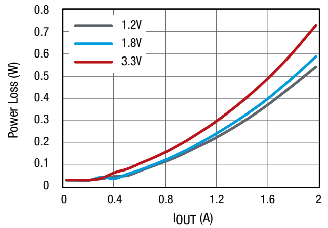
Figure 21. Channel 1 Power Loss at f sw = 500kHz, V IN = 12V, No Airflow
