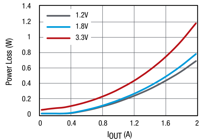
Figure 25. Channel 2 Power Loss at f sw = 500kHz, V IN = 5V, No Airflow
