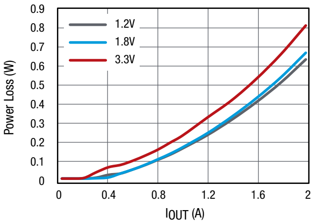
Figure 22. Channel 2 Power Loss at f sw = 500kHz, V IN = 12V, No Airflow
