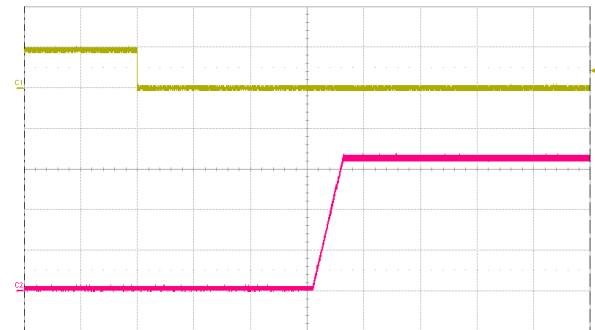
Fig. 10: Turn-on transient at full rated load current (resistive) plus 10,000 \mu\text{F} at V_{in} = 48\text{ V} , triggered via ON/OFF pin. Top trace: ON/OFF signal (5 V/div.). Bottom trace: output voltage (1 V/div.). Time scale: 20 ms/div.
