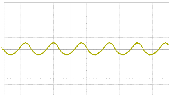
Fig. 15: Input reflected ripple current, i_c (1 A/div.), measured at input terminals at full rated load current and V_{in} = 48 \text{ V} . Refer to Fig. 14 for test setup. Time scale: 2 \mu\text{s}/\text{div} .
