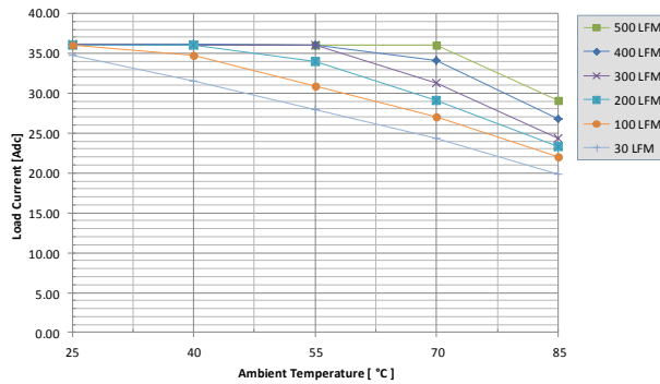
Fig. 2: Power derating vs. ambient air temperature and airflow rates for UIE48T36033 converter w/o baseplate
