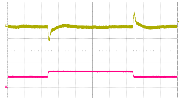
Fig. 12: Output voltage response to load current step change (18A – 27A – 18A) at V_{in} = 48\text{ V} . Top trace: output voltage (200 mV/div.). Bottom trace: load current (20 A/div.). Current slew rate: 1 A/ \mu\text{s} . C_o = 1\text{ }\mu\text{F} ceramic + 10,000 \mu\text{F} + 10 \mu\text{F} tantalum. Time scale: 200 \mu\text{s} /div.
