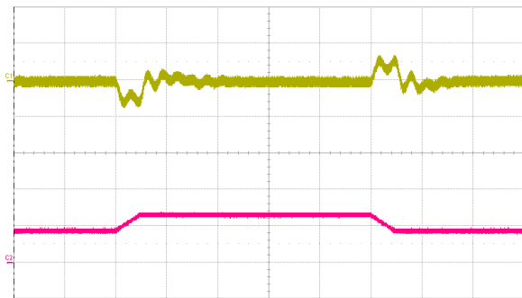
Fig. 11: Output voltage response to load current step change (18A – 27A – 18A) at V_{in} = 48\text{ V} . Top trace: output voltage (200 mV/div.). Bottom trace: load current (20 A/div.). Current slew rate: 0.1 A/ \mu\text{s} . C_o = 1\text{ }\mu\text{F} ceramic + 10 \mu\text{F} tantalum. Time scale: 200 \mu\text{s} /div.
