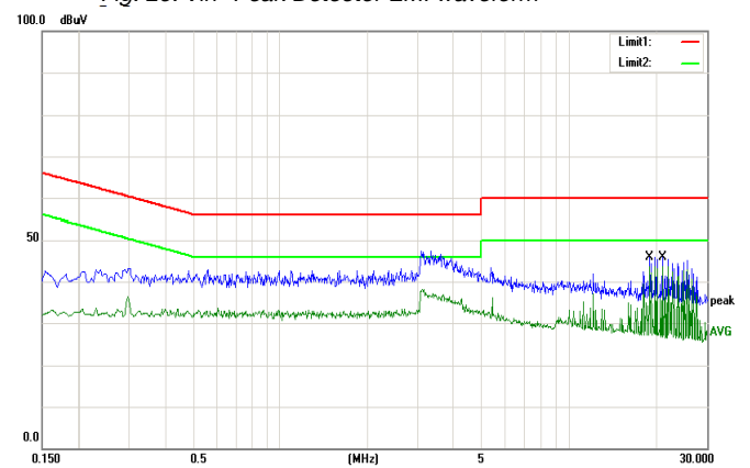
Fig. 20: Vin- Peak Detector EMI waveform
