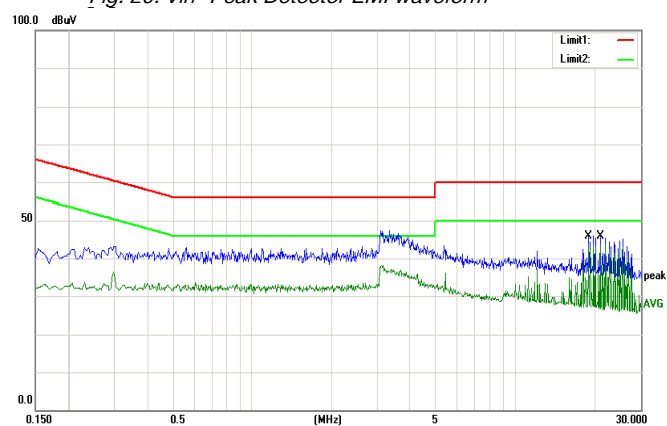
Fig. 20: Vin- Peak Detector EMI waveform
