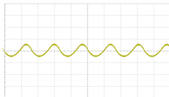
Fig. 16: Input reflected ripple current, i_s (50 mA/div.), measured through 10\text{ }\mu\text{H} at the source at full rated load current and V_{in} = 48\text{ V} . Refer to Fig. 14 for test setup. Time scale: 2\text{ }\mu\text{s/div.}
