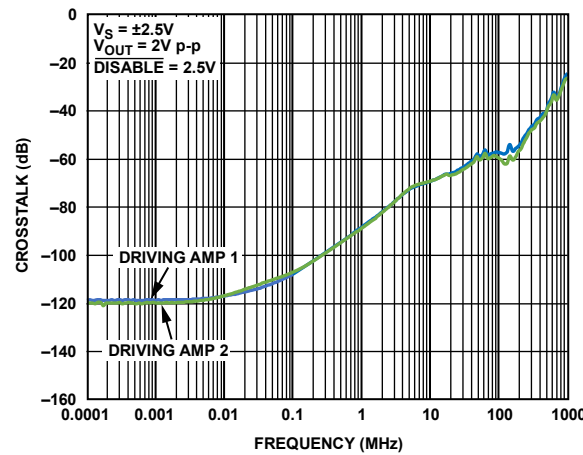
Figure 36. Crosstalk vs. Frequency
