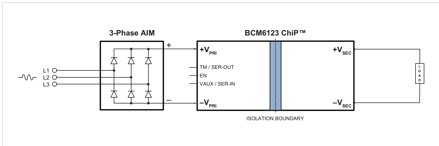
3-phase AC to point-of-load (3-phase AIM™ + BCM6123xD1E5135yzz)
