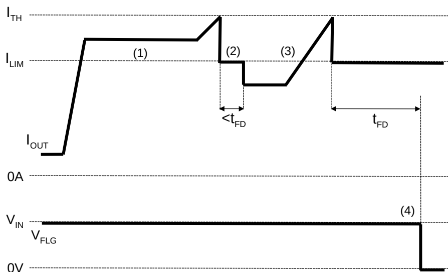
R5524x002A/002B and R5524N004A (Constant Current Type) Timing Chart
