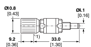
Part No. 2-1393670-2 ♦ Coupling Type A, B 2 , F 2
