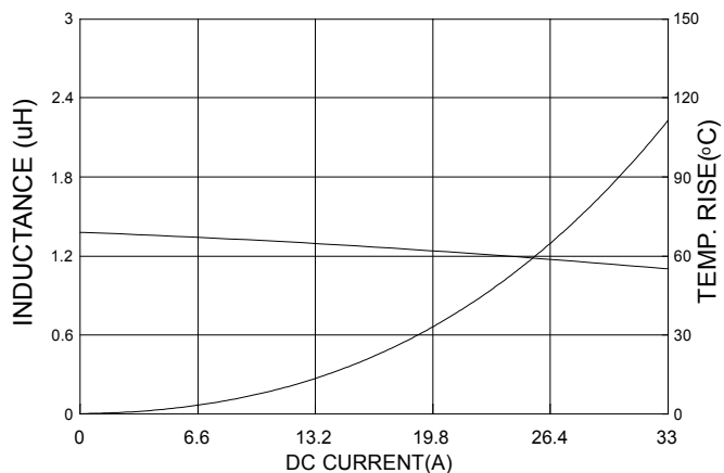
PA4342.152NLT
