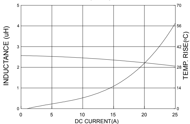
PA4342.252NLT
