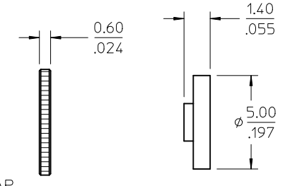
INSULATOR
