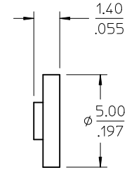
INSULATOR
